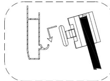
Top Wheels
